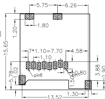
RECOMMENDED P.C.B HOLE LAYOUT COMPONENT SIDE VIEW(TOLERANCE: \pm 0.05 )
