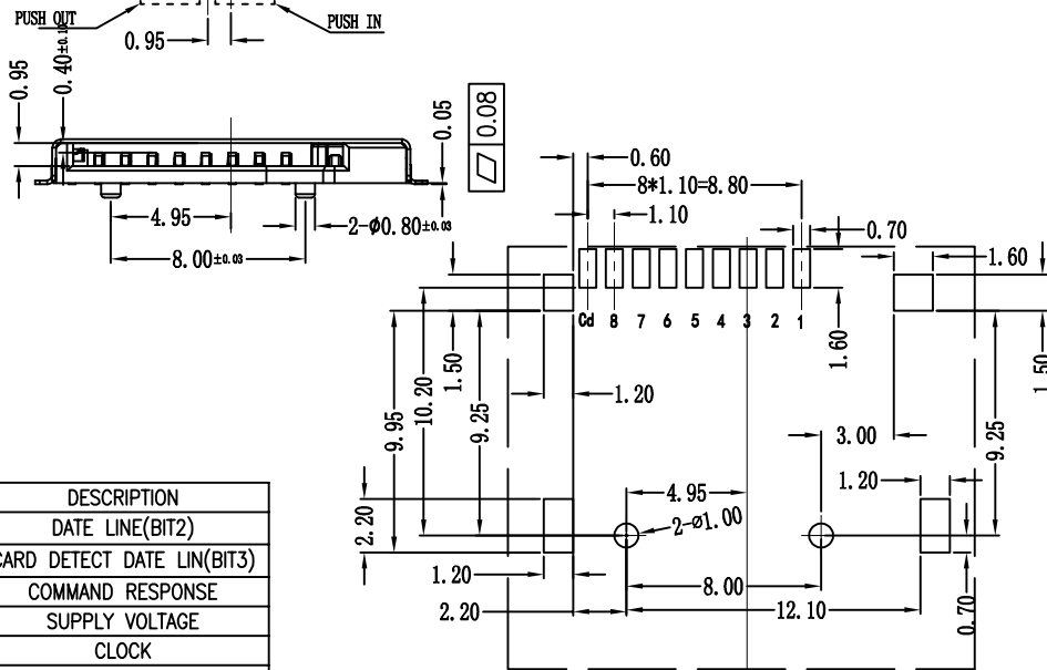
RECOMMENDED P.C.B HOLE LAYOUT COMPONENT SIDE VIEW(TOLERANCE: +/-0.05)
